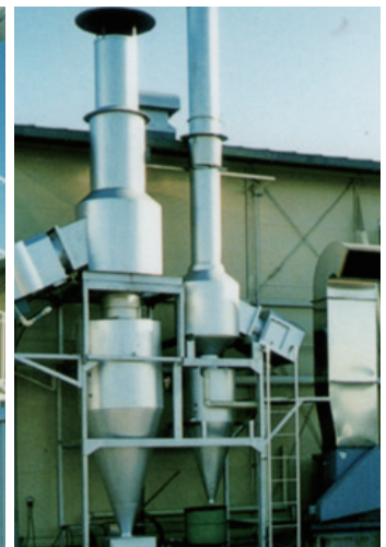
Example installation of type for both exhaust and cooling
